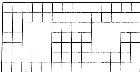
FIG. 1. Two adjacent blocks for d_y = 2 .
